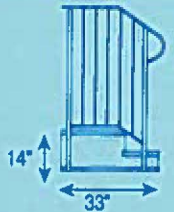
STOOP (10027S)
