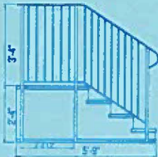
STOOP (1004736S)
