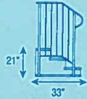
STEPS (10037)
